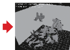
Bulk parts supply state is repeated with physical simulation
